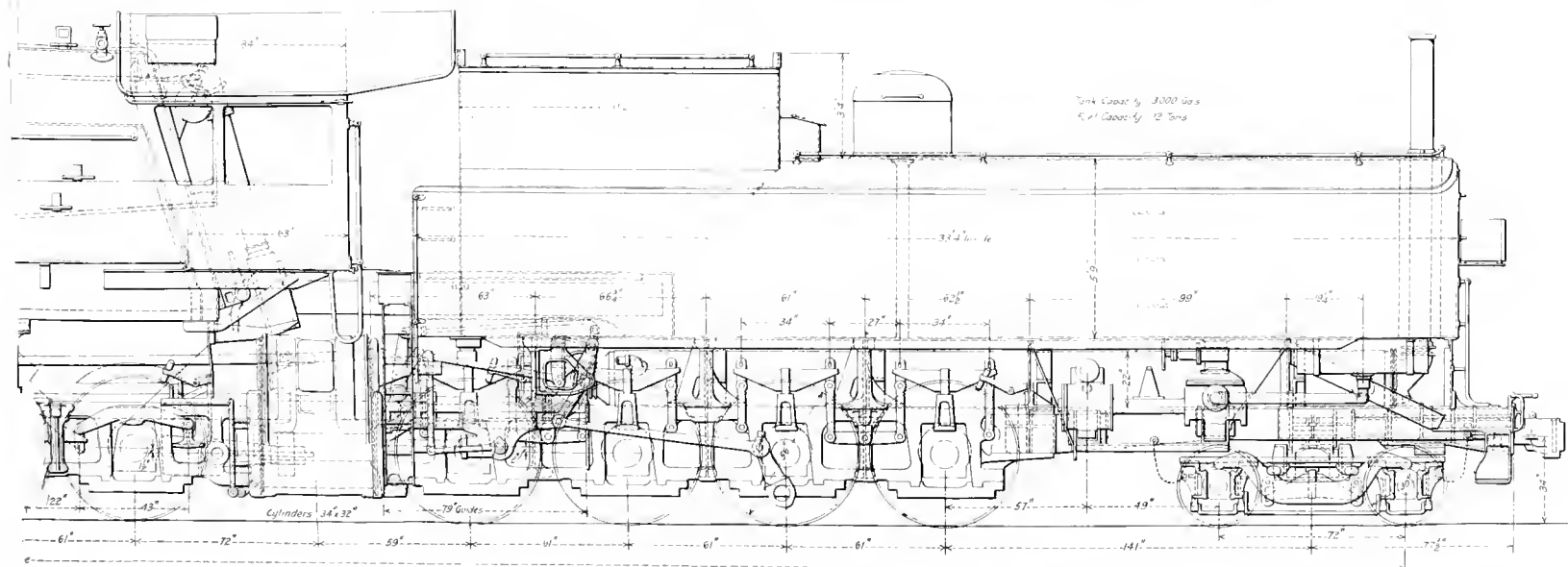
Railway; Total Weight, 844,000 lb.; Tractive Effort, 166,300 lb.
